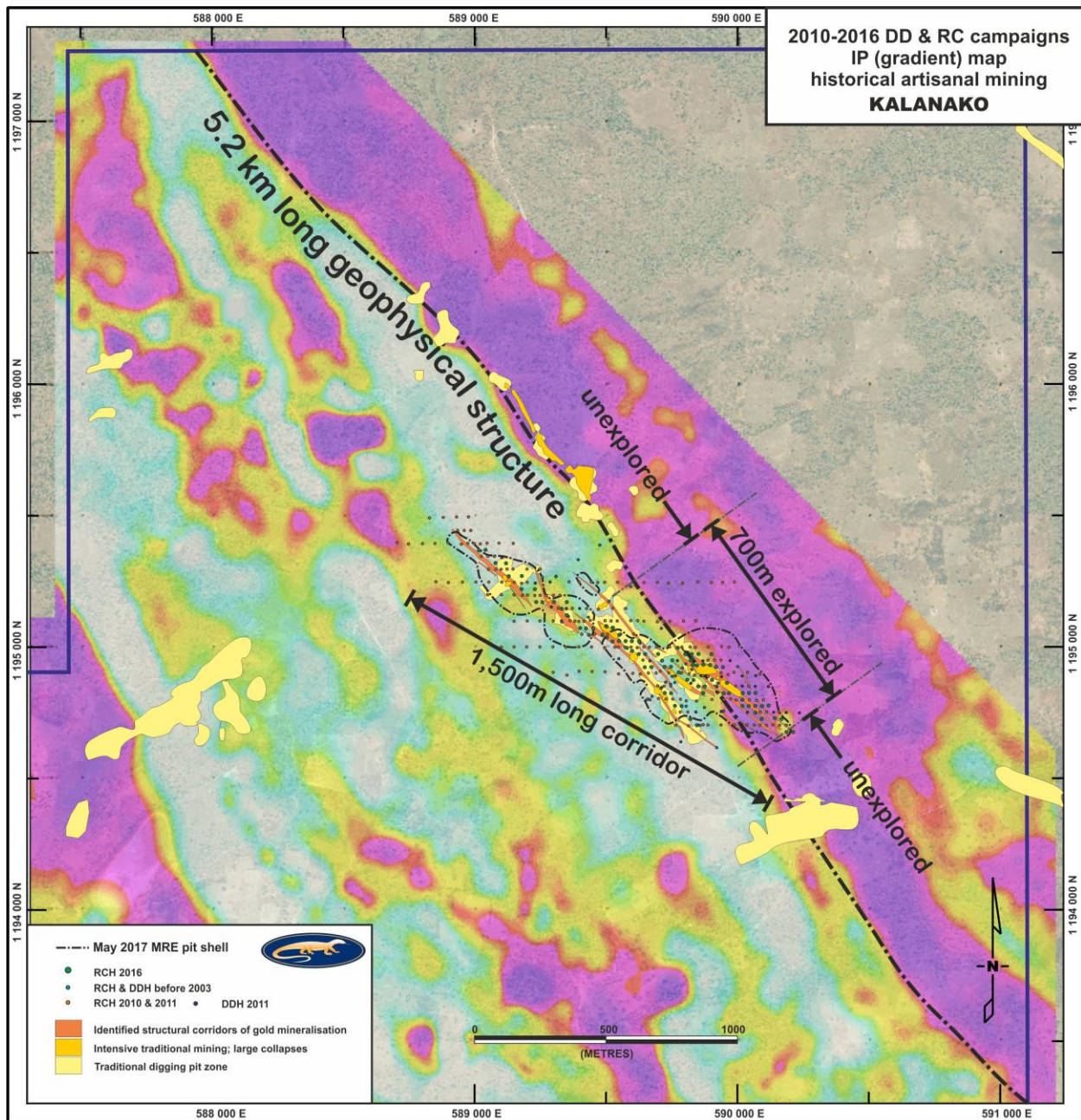
Figure 5: Kalanako drilled area and resources on the 5.2km long geophysical trend.
