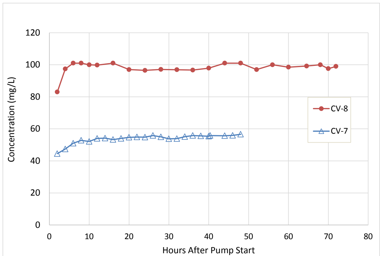
Figure 1 - Lithium concentrations in brine extracted during pumping tests at CV-7 and CV-8
