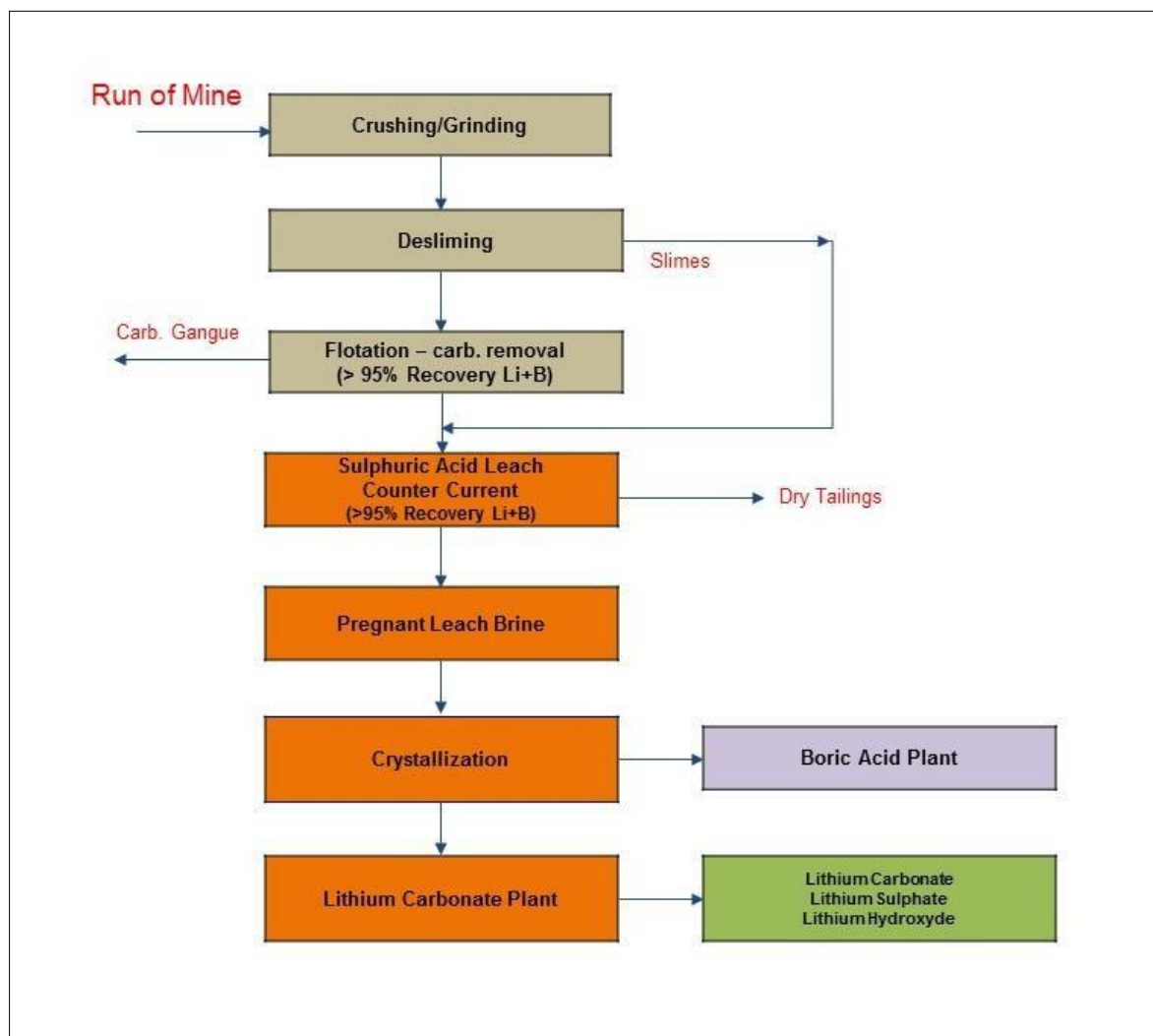
Figure 3. Rhyolite Ridge simplified conceptual flowsheet
