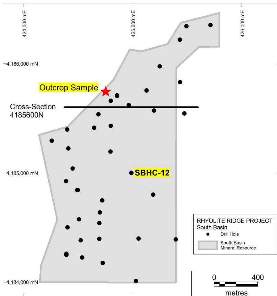
Figure 4. South Basin Resource area showing location of metallurgical samples from outcrop and diamond core hole SBHC-12.
