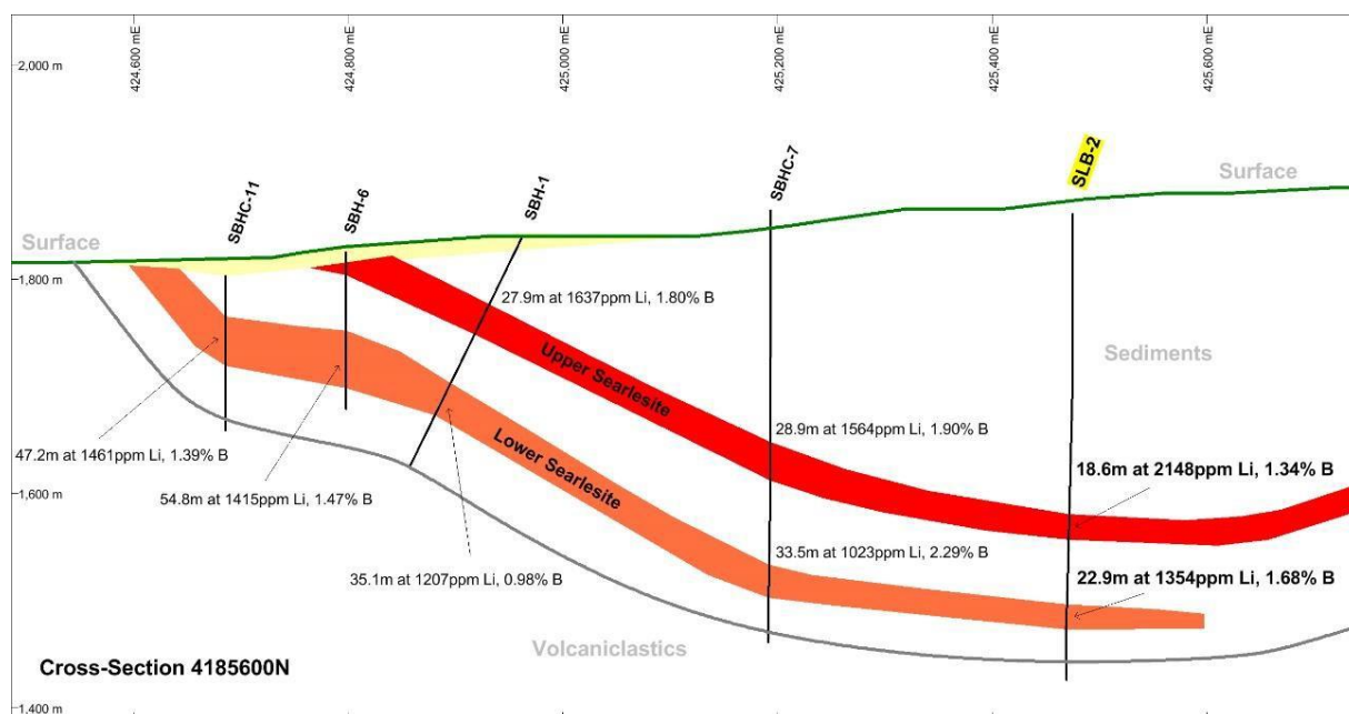
Figure 5. South Basin cross-section 4185600N showing the upper and lower searlesite (Li-B) zones. The upper searlesite zone contains the 63Mt of the 65Mt high-grade Resource.
