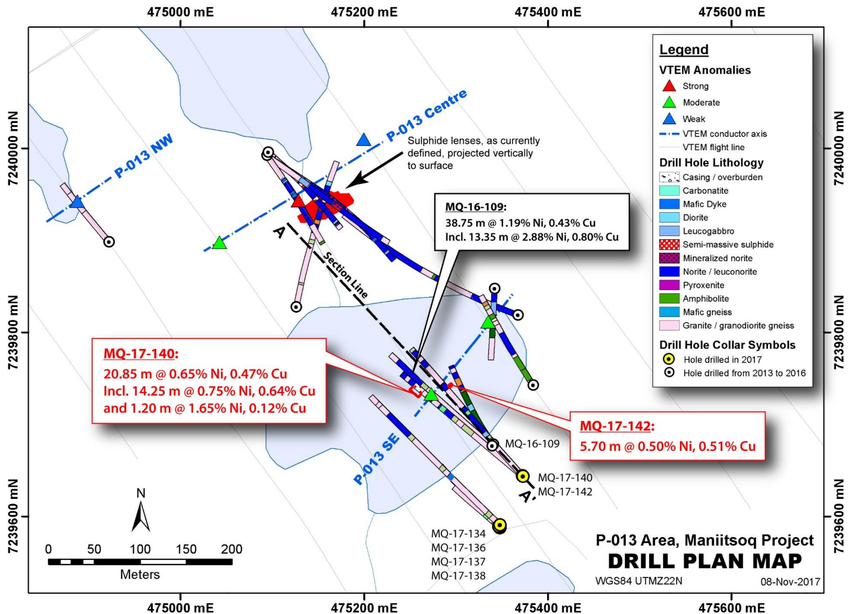
Figure 2: Plan map of the P-013 area showing locations of diamond drill holes, interpreted VTEM conductors and selected assay composites discussed in this news release. 2017 hole collars are coloured yellow.
