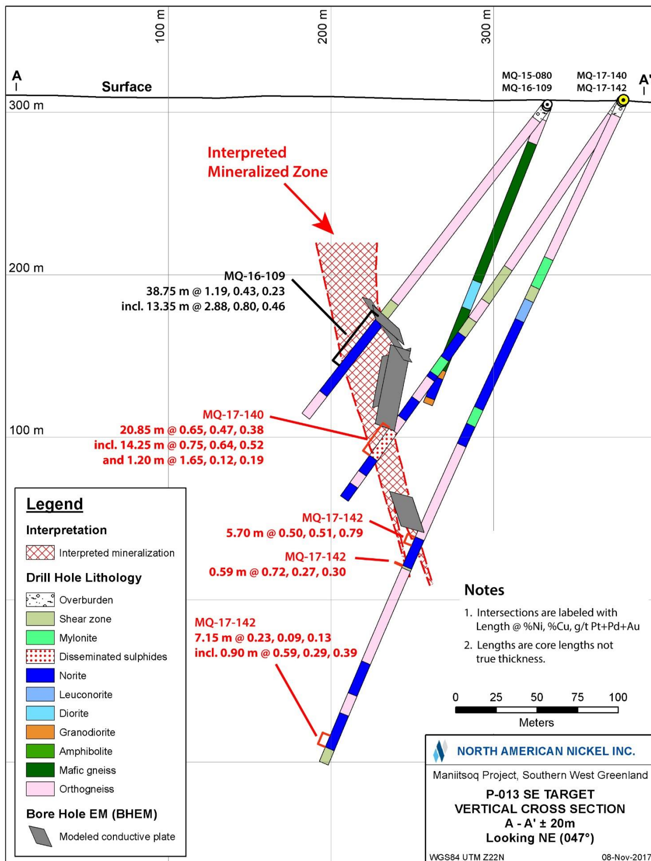
Figure 3: Vertical cross section through the P-013 SE mineralized zone. The azimuth of the section is 137° and it looks N047° E.
