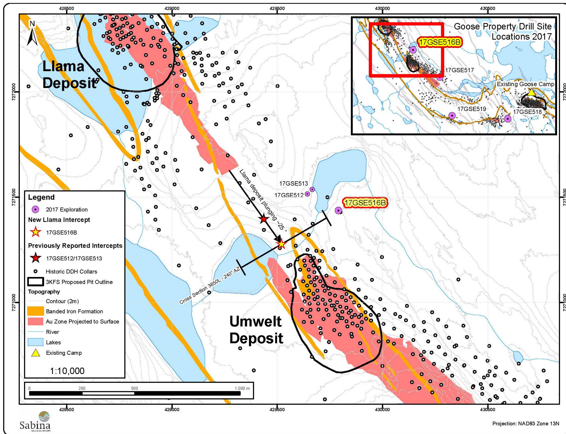
Figure 1 – Plan map of 2017 drilling with detail for the Llama-Umwelt mineralization trend.
