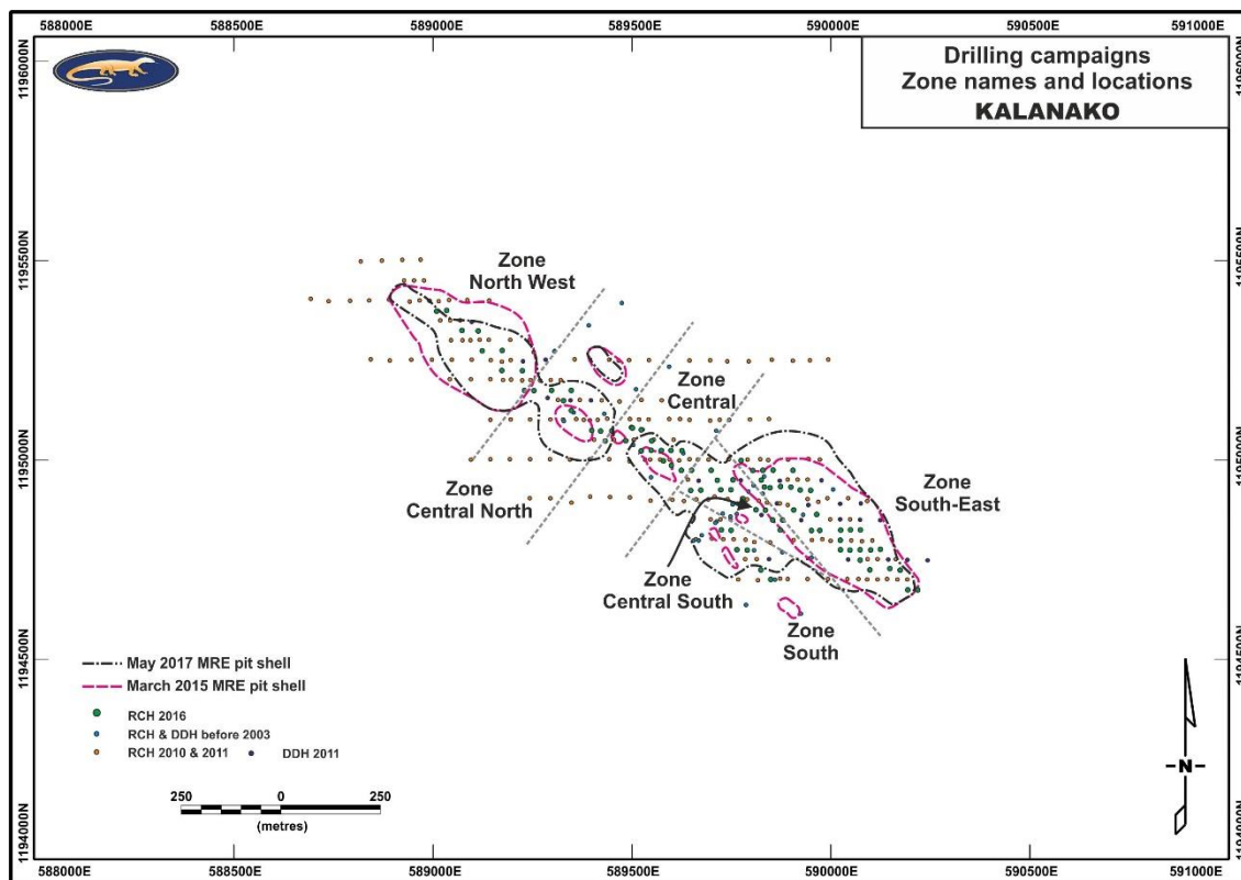
Figure 1: Kalanako Drilling pattern, zones and pit shells.
