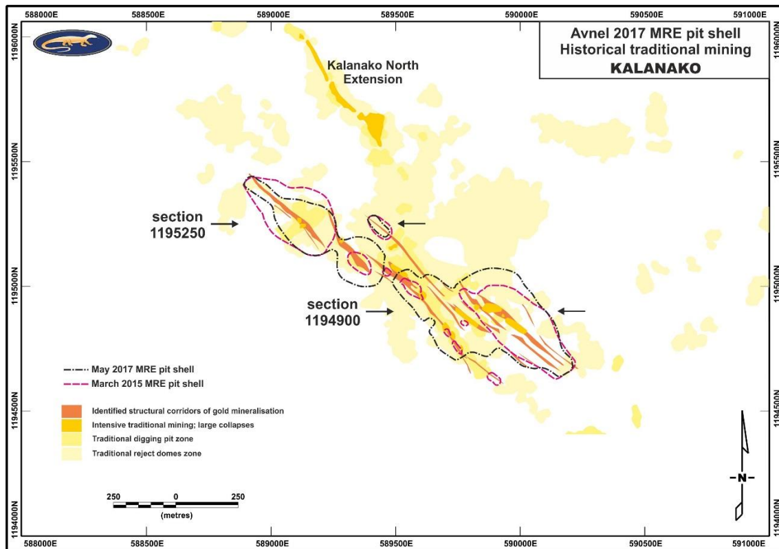
Figure 2: Kalanako mineralisations, historical traditional mining and resource pit shells.
