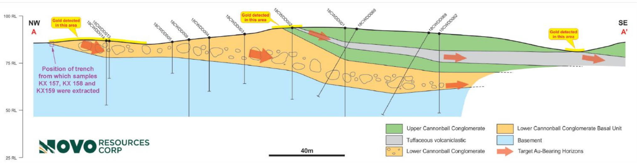
(Figure 4: Cross section showing the stratigraphy at the Powerline showing and the position of the trench from which samples KX157 and KX158 originate. The position of gold detector strikes is also shown. Note the two gold-bearing horizons, one at the bottom of the Lower Cannonball conglomerate and the other at the bottom of the Upper Cannonball conglomerate. The upper gold-bearing horizon may correlate with that found approximately 2 km northeast at Purdy's Reward.)
